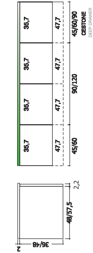
BASI SOSPESE LIVING HANGING LIVING BASE UNITS
